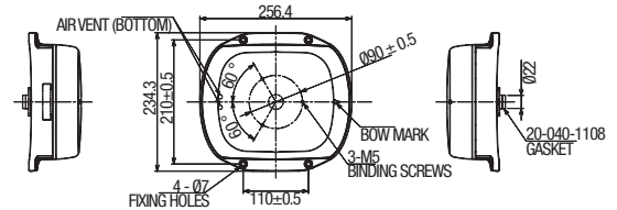
SCX-20 w/ roof mount 1.4 kg (3.0 lbs)
