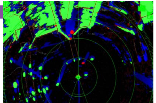
Model FR-12 12" Color LCD Marine Radar Display
